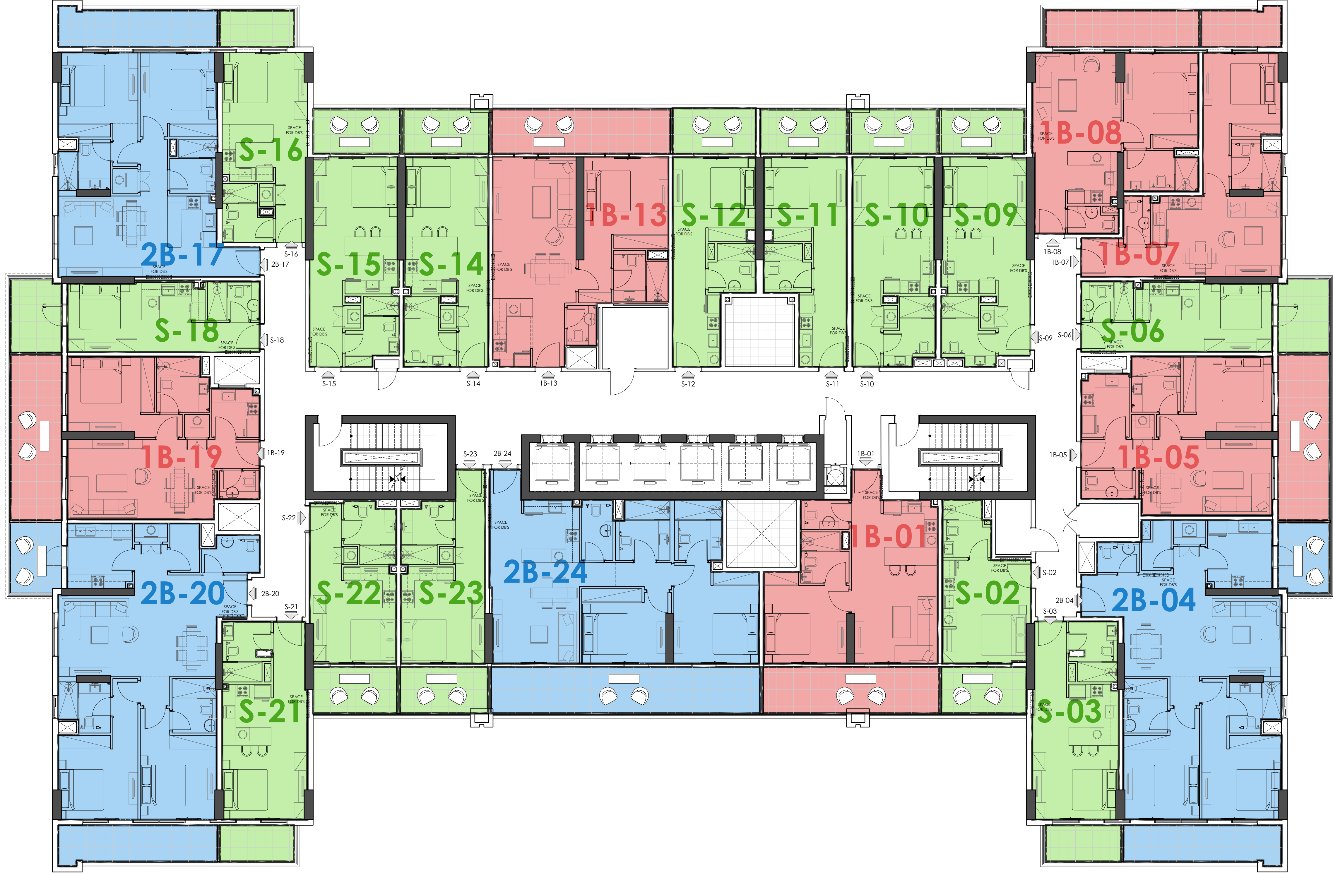
3RD-9TH & 11TH-13TH FLOOR PLAN
